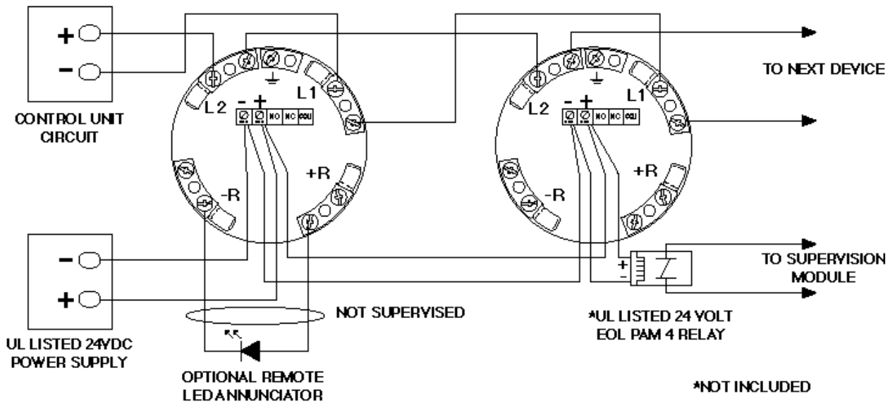
Wiring Schematic for MB-RLY-XP95 Relay Base
